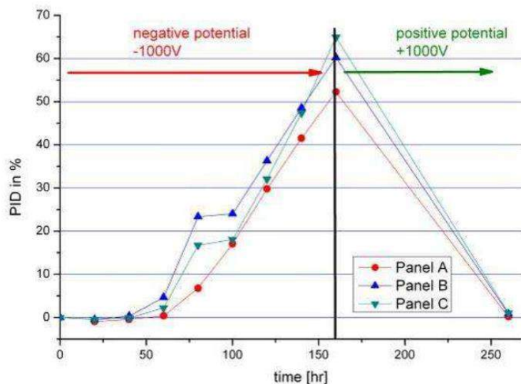
Figure 3: PID and recovery by reverse potential. [1]
